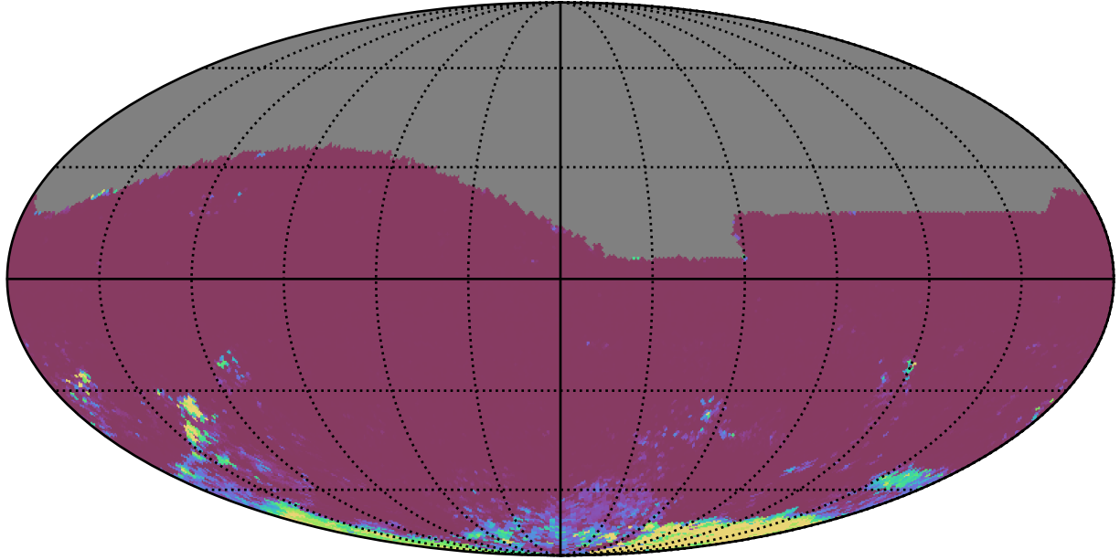
too_elab_r256_d2_ugrizy_v3.4_10yrs All sky ri bands: 75th Percentile Intranight Timespan
