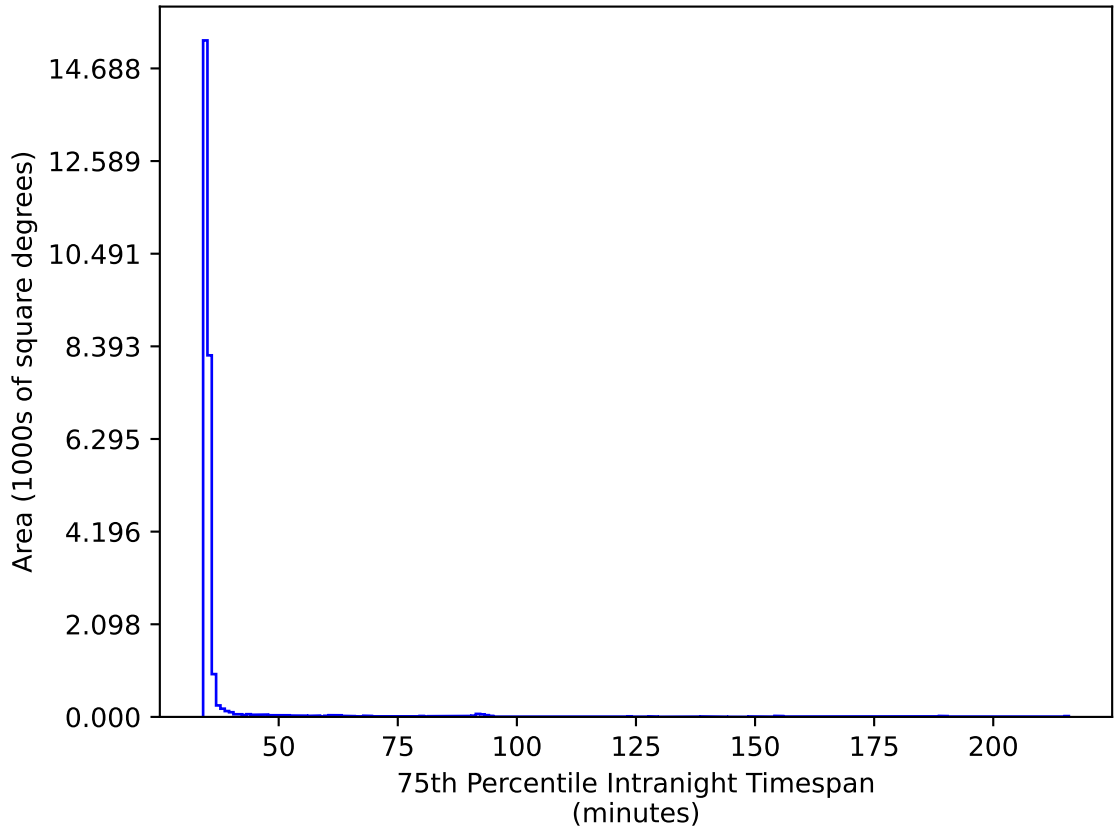
too_elab_r256_d2_ugrizy_v3.4_10yrs All sky ri bands: 75th Percentile Intranight Timespan
