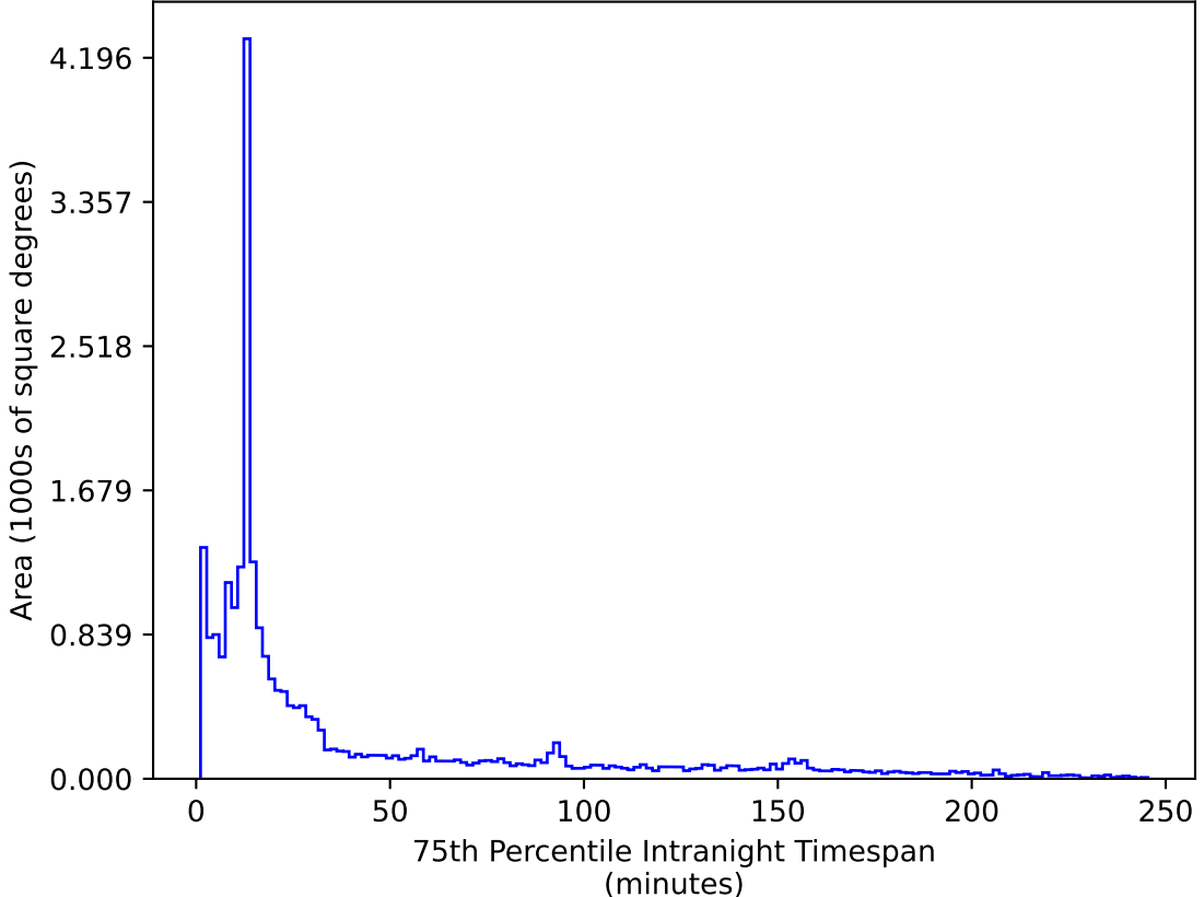
too_elab_r256_d2_ugrizy_v3.4_10yrs All sky i band: 75th Percentile Intranight Timespan
