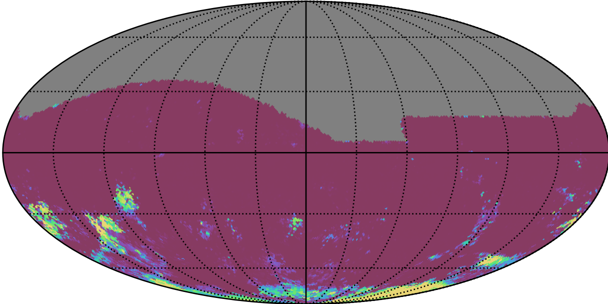
too_elab_r256_d2_ugrizy_v3.4_10yrs All sky gr bands: 75th Percentile Intranight Timespan
