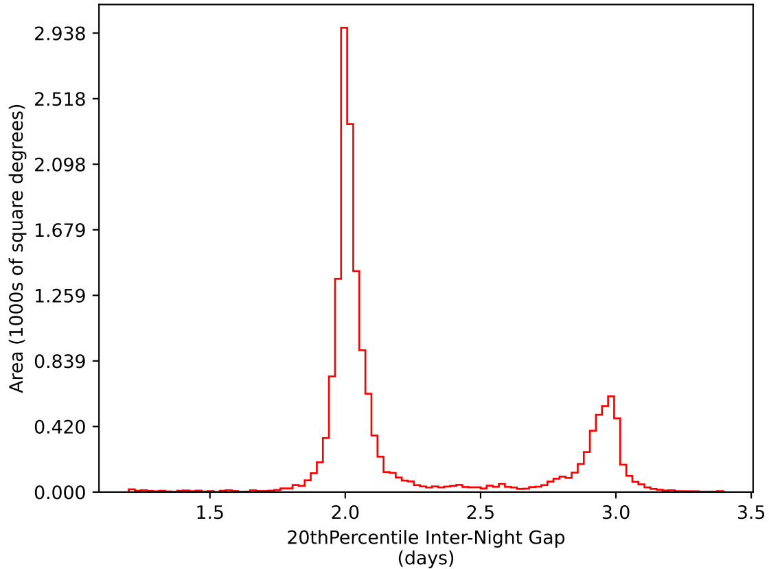
too_elab_r256_d2_ugrizy_v3.4_10yrs WFD i band: 20thPercentile Inter-Night Gap
