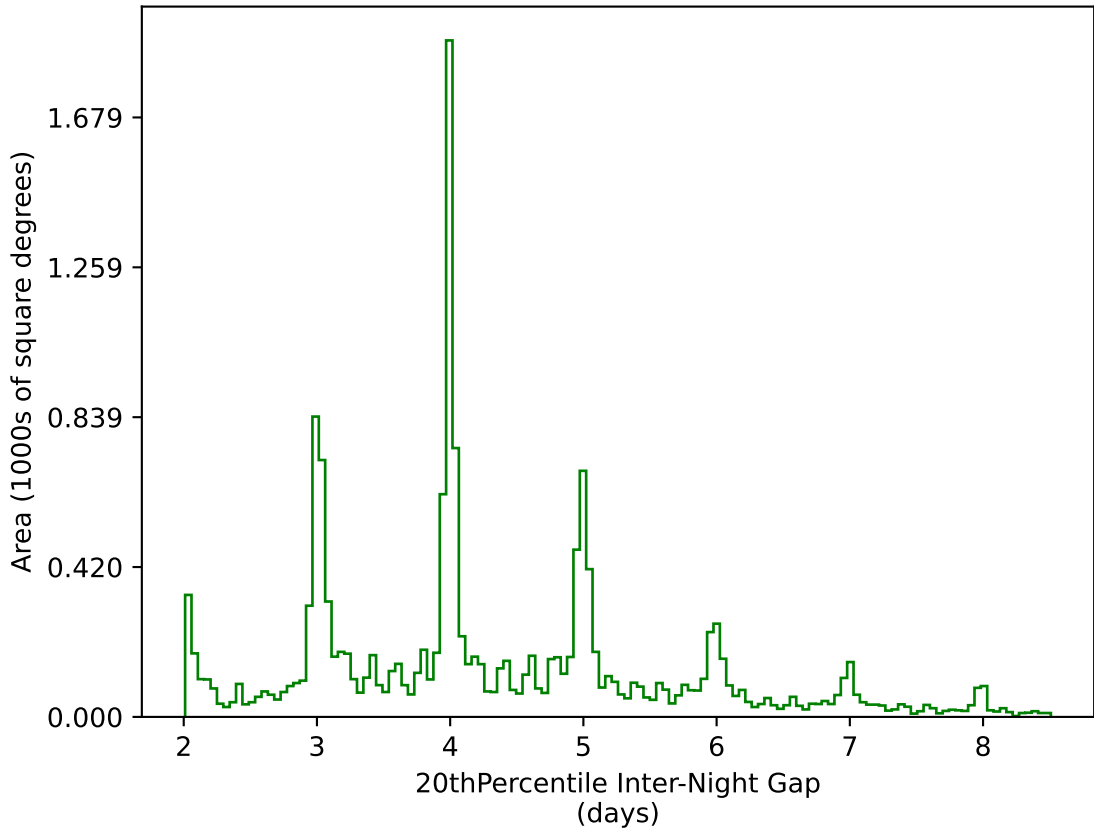
too_elab_r256_d2_ugrizy_v3.4_10yrs WFD g band: 20thPercentile Inter-Night Gap
