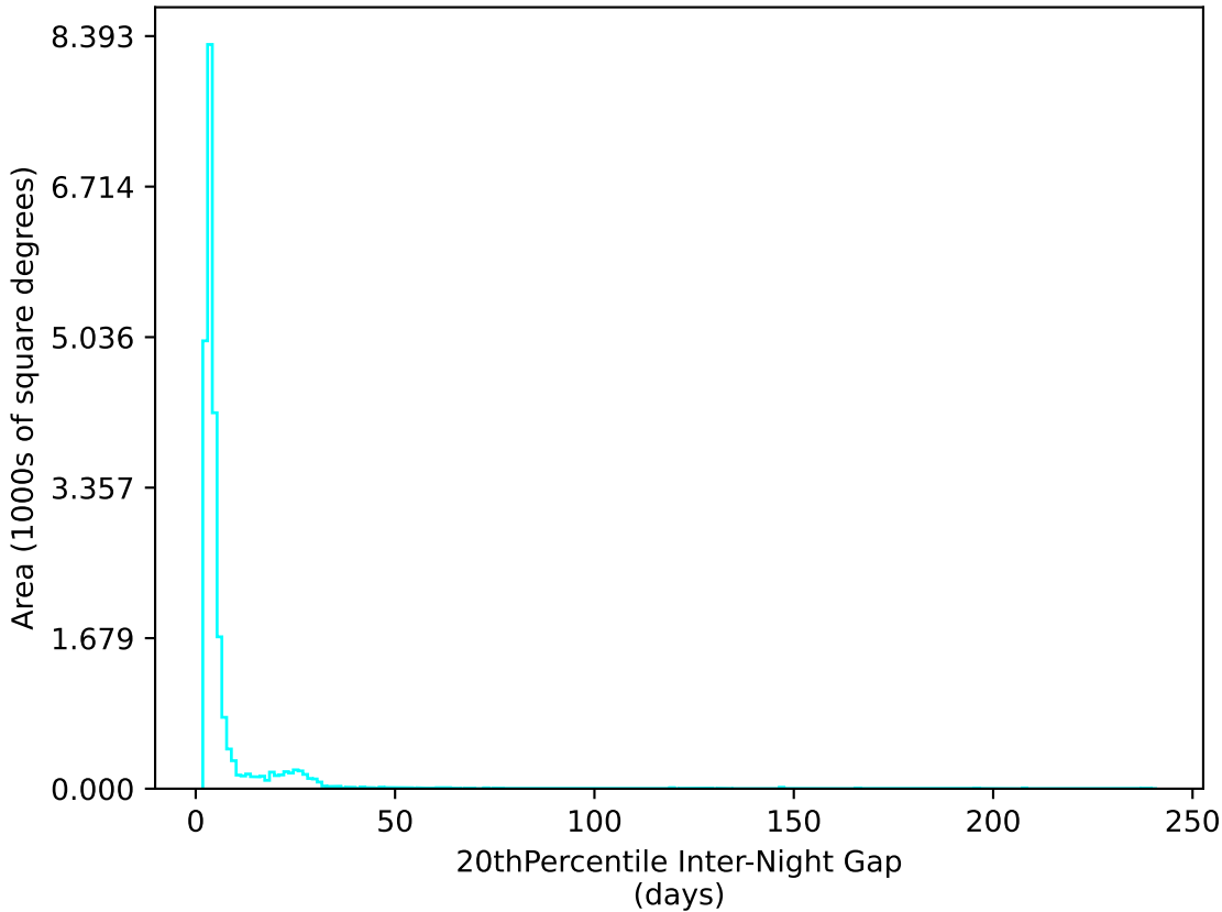
too_elab_r256_d2_ugrizy_v3.4_10yrs All sky u band: 20thPercentile Inter-Night Gap
