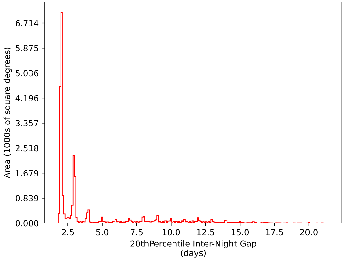
too_elab_r256_d2_ugrizy_v3.4_10yrs All sky i band: 20thPercentile Inter-Night Gap
