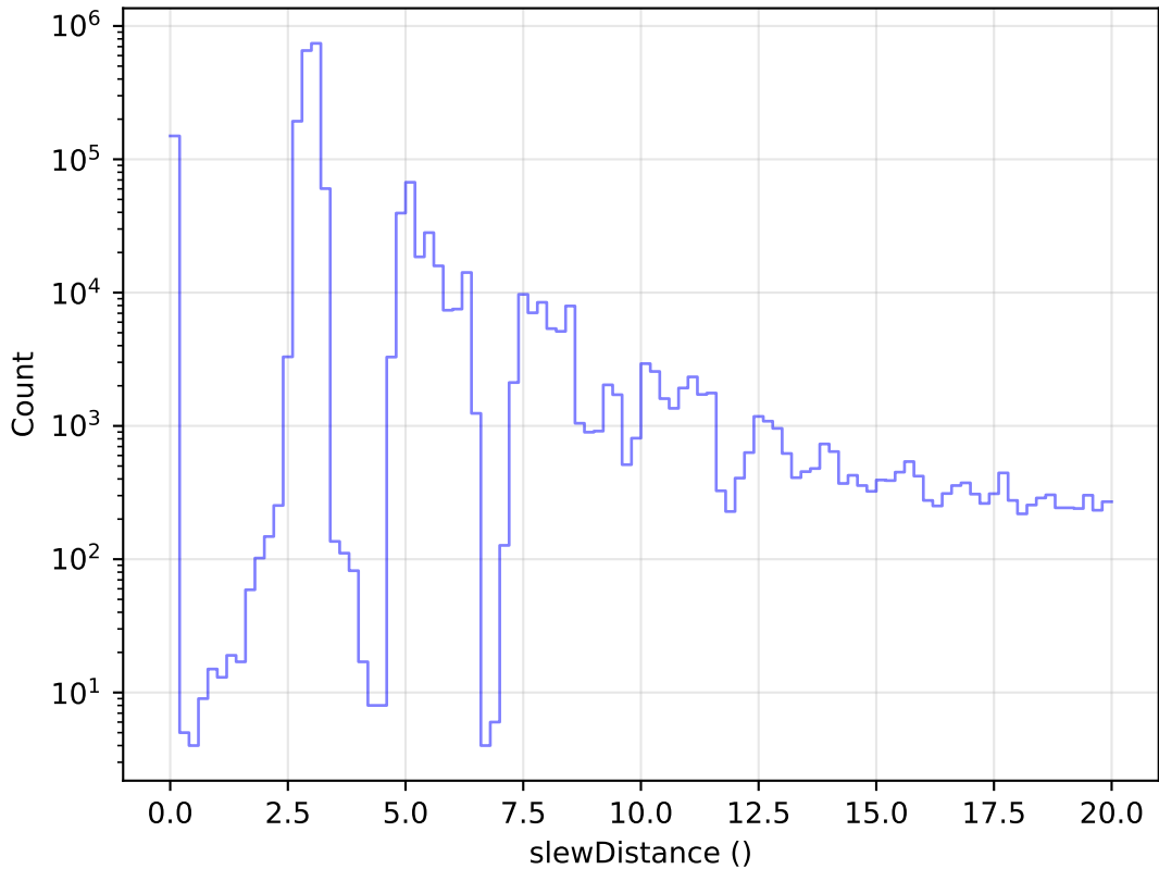
too_elab_r256_d2_ugrizy_v3.4_10yrs All visits: Zoom Slew Distance Histogram
