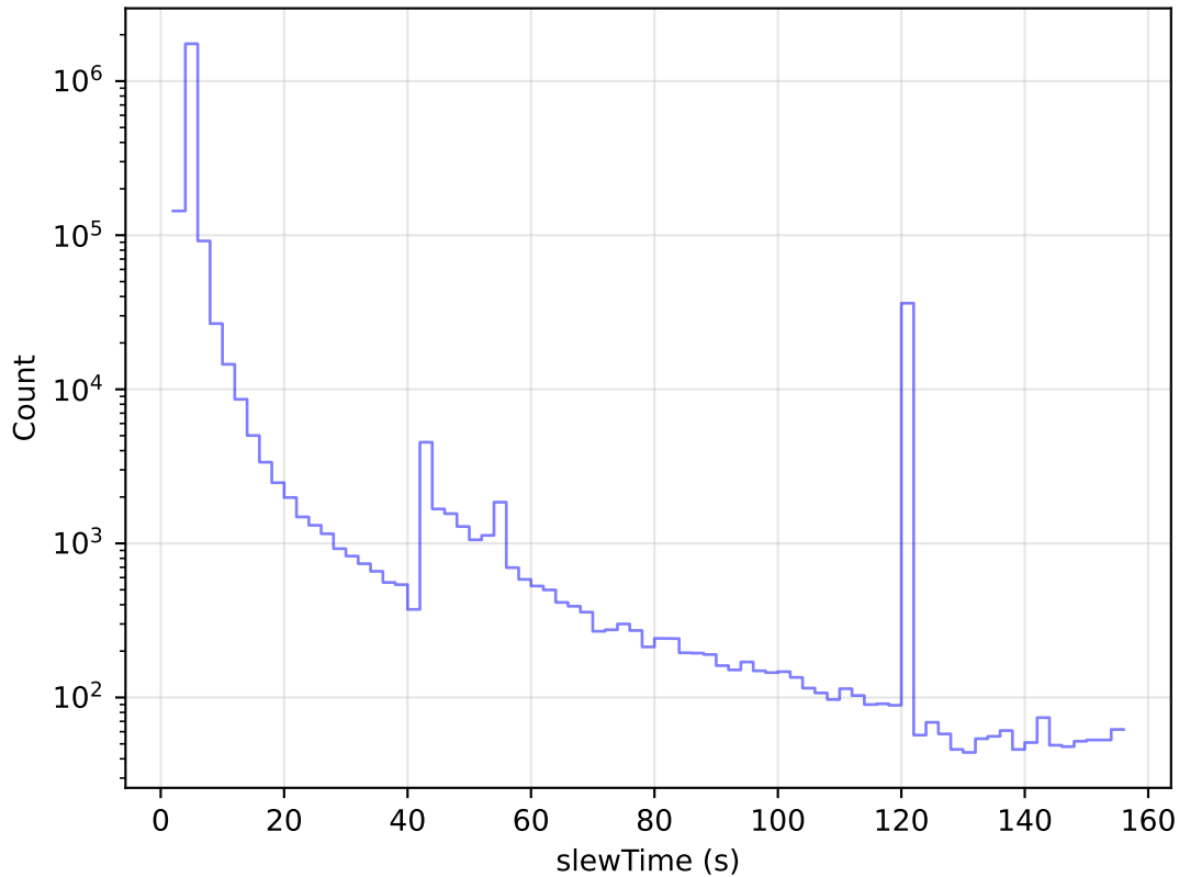
too_elab_r256_d2_ugrizy_v3.4_10yrs All visits: Slew Time Histogram
