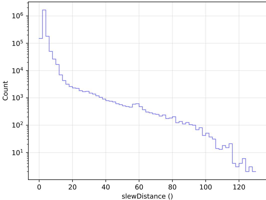
too_elab_r256_d2_ugrizy_v3.4_10yrs All visits: Slew Distance Histogram
