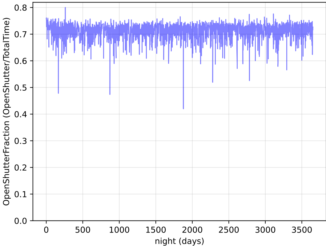
too_elab_r256_d2_ugrizy_v3.4_10yrs : OpenShutterFraction
