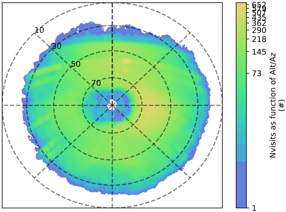
too_elab_r256_d2_ugrizy_v3.4_10yrs u: Nvisits as function of Alt/Az
