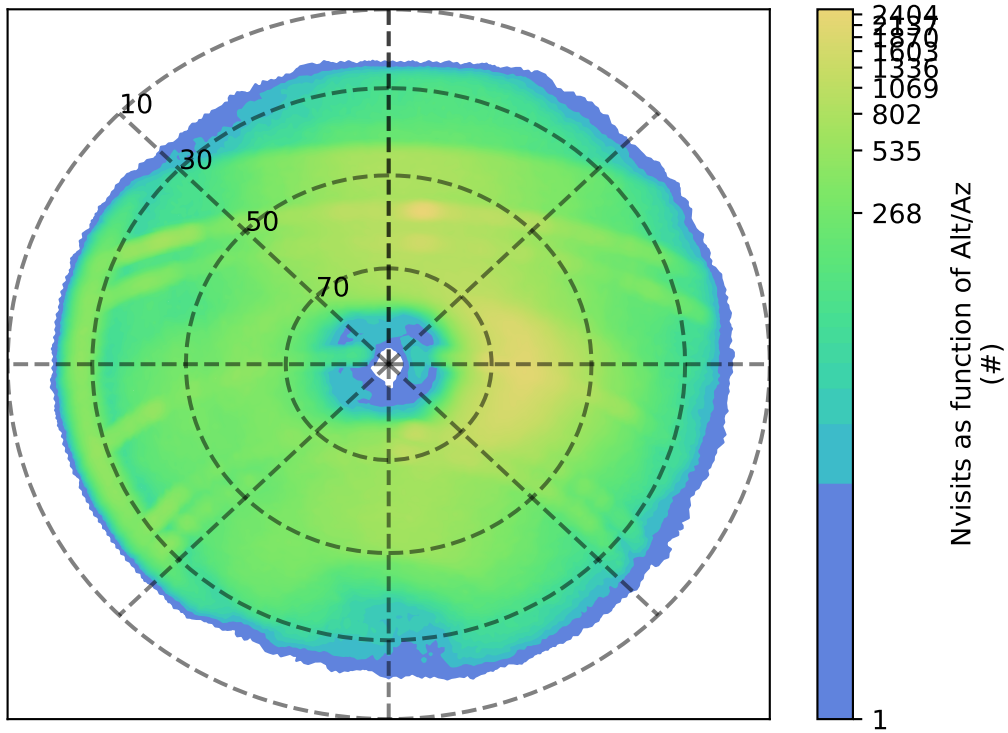
too_elab_r256_d2_ugrizy_v3.4_10yrs r: Nvisits as function of Alt/Az
