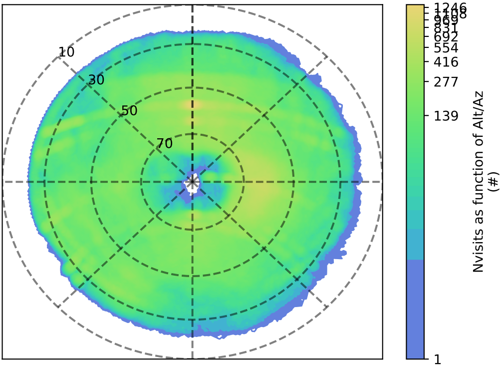
too_elab_r256_d2_ugrizy_v3.4_10yrs g: Nvisits as function of Alt/Az
