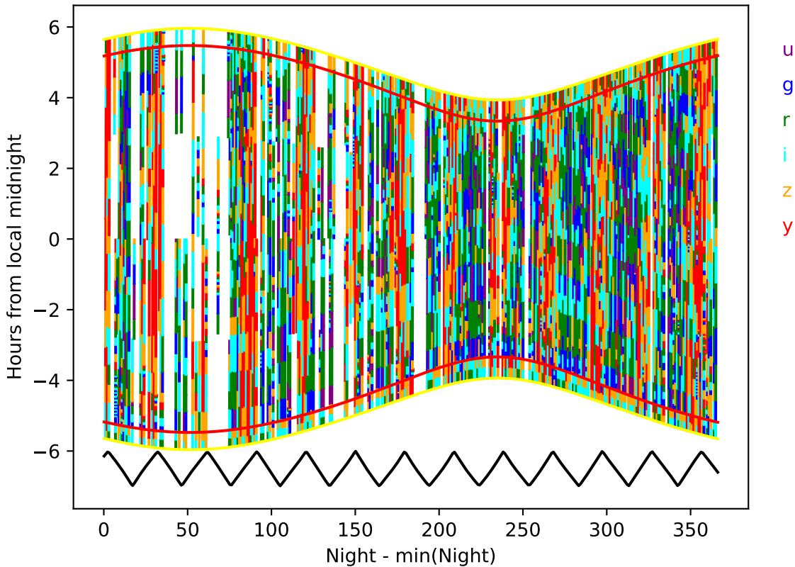
too_elab_r256_d2_ugrizy_v3.4_10yrs year 9-10: Hourglass
