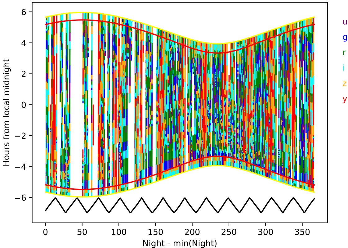
too_elab_r256_d2_ugrizy_v3.4_10yrs year 8-9: Hourglass
