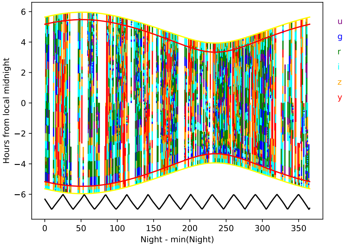
too_elab_r256_d2_ugrizy_v3.4_10yrs year 7-8: Hourglass
