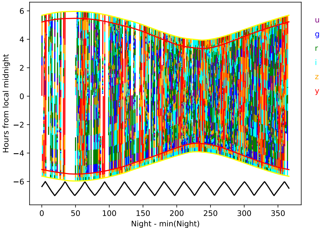
too_elab_r256_d2_ugrizy_v3.4_10yrs year 6-7: Hourglass
