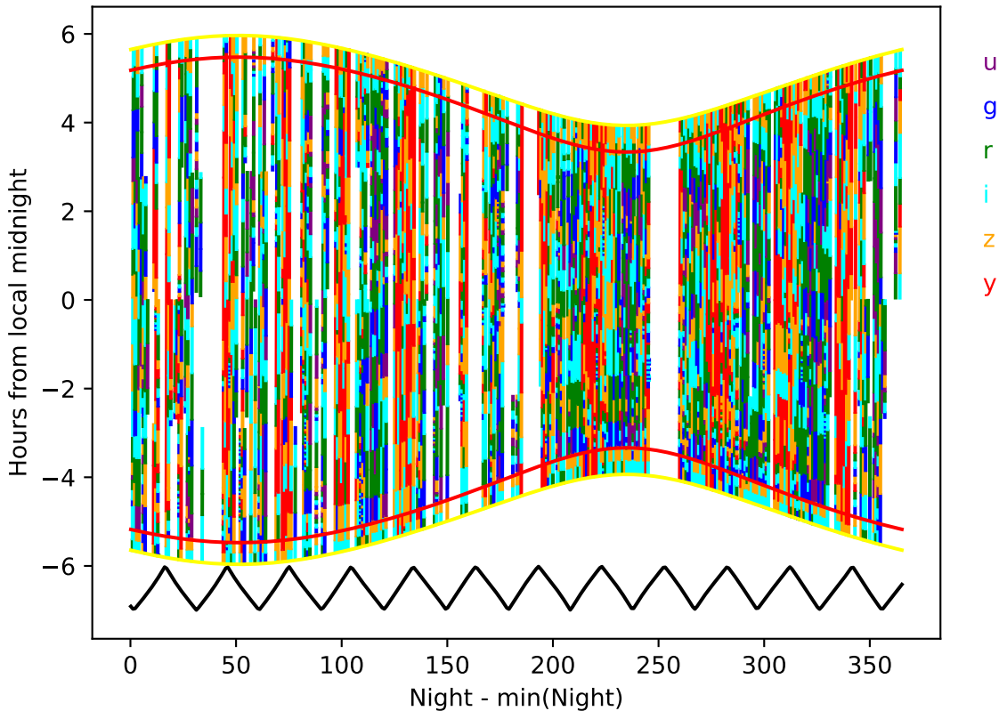
too_elab_r256_d2_ugrizy_v3.4_10yrs year 5-6: Hourglass
