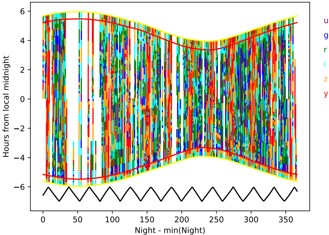
too_elab_r256_d2_ugrizy_v3.4_10yrs year 3-4: Hourglass
