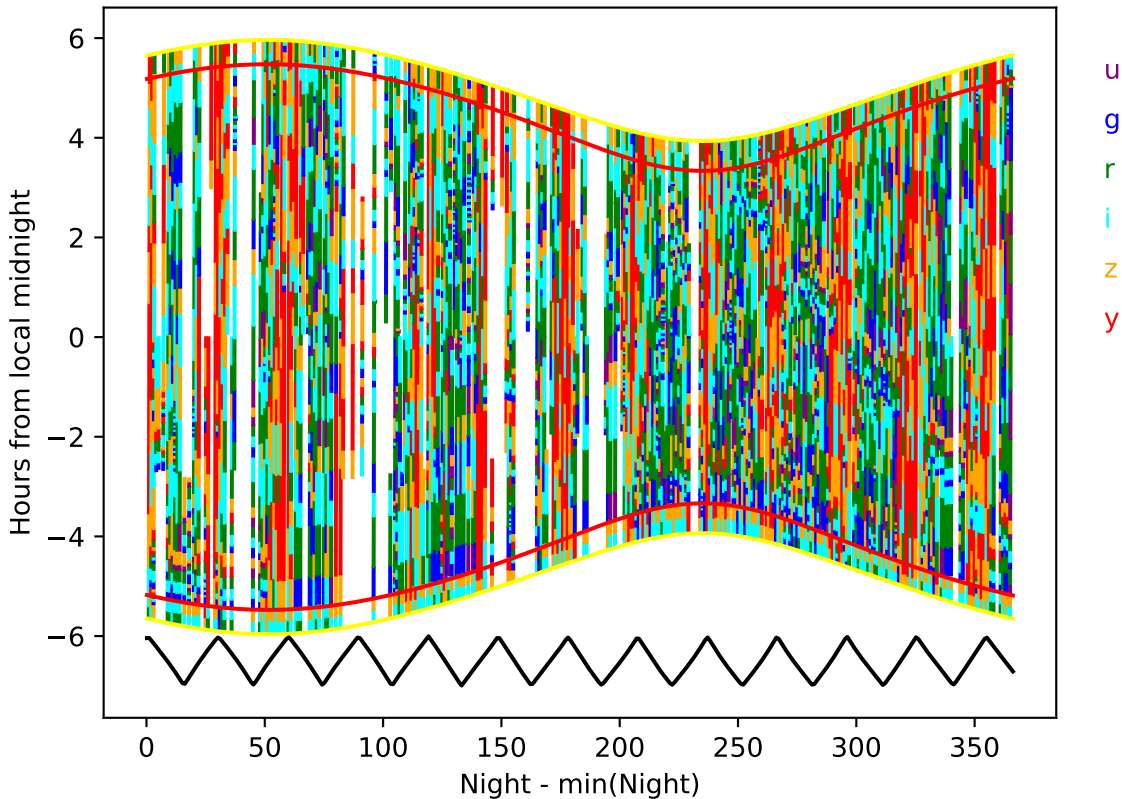
too_elab_r256_d2_ugrizy_v3.4_10yrs year 1-2: Hourglass
