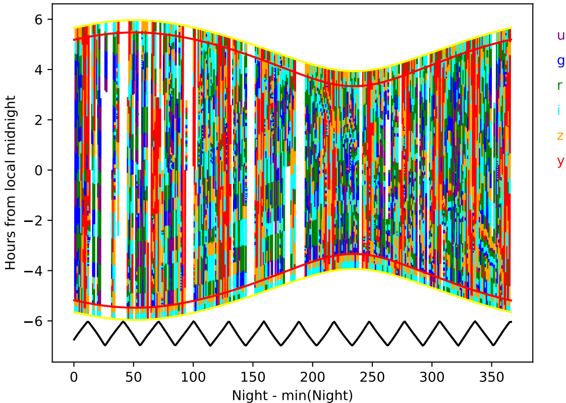
too_elab_r256_d2_ugrizy_v3.4_10yrs year 0-1: Hourglass
