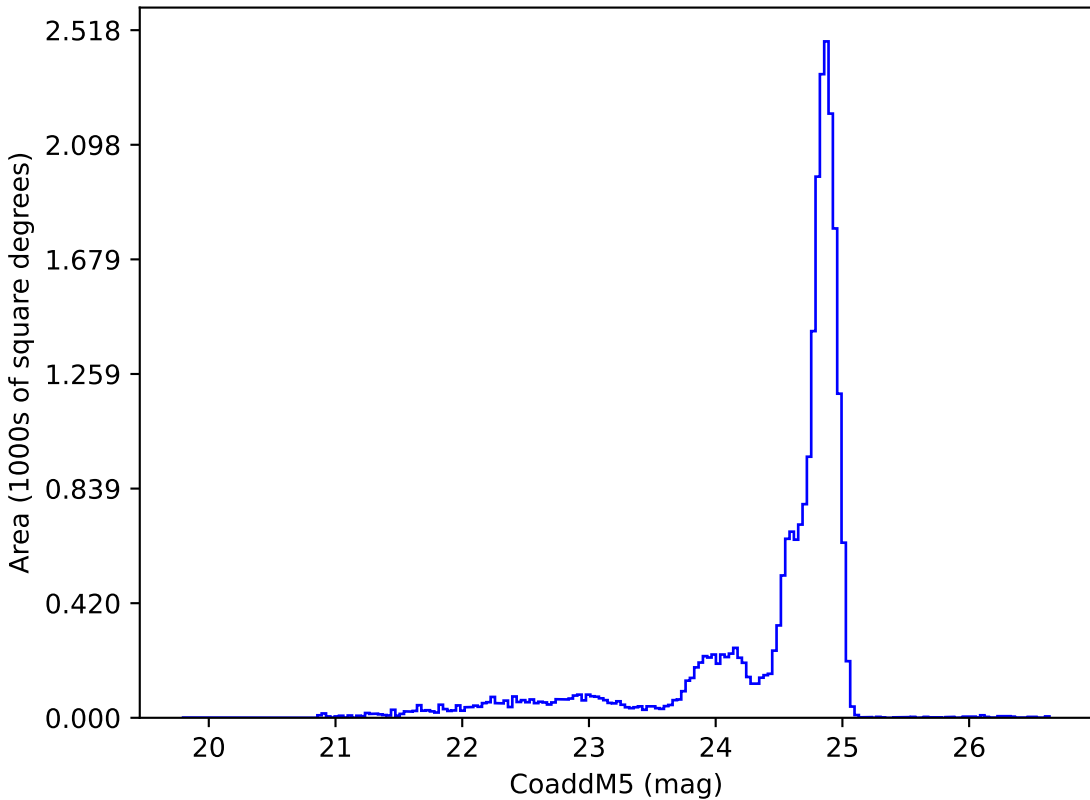
too_elab_r256_d2_ugrizy_v3.4_10yrs y: CoaddM5
