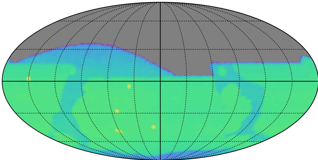
too_elab_r256_d2_ugrizy_v3.4_10yrs r: CoaddM5
