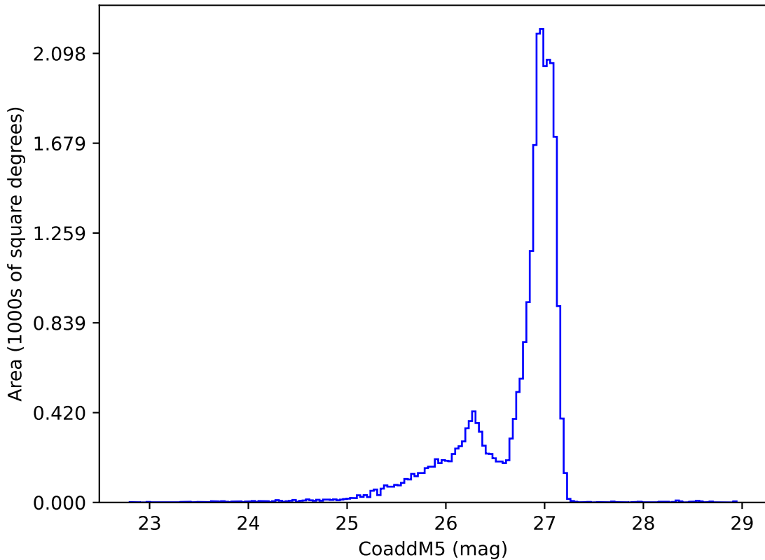
too_elab_r256_d2_ugrizy_v3.4_10yrs r: CoaddM5
