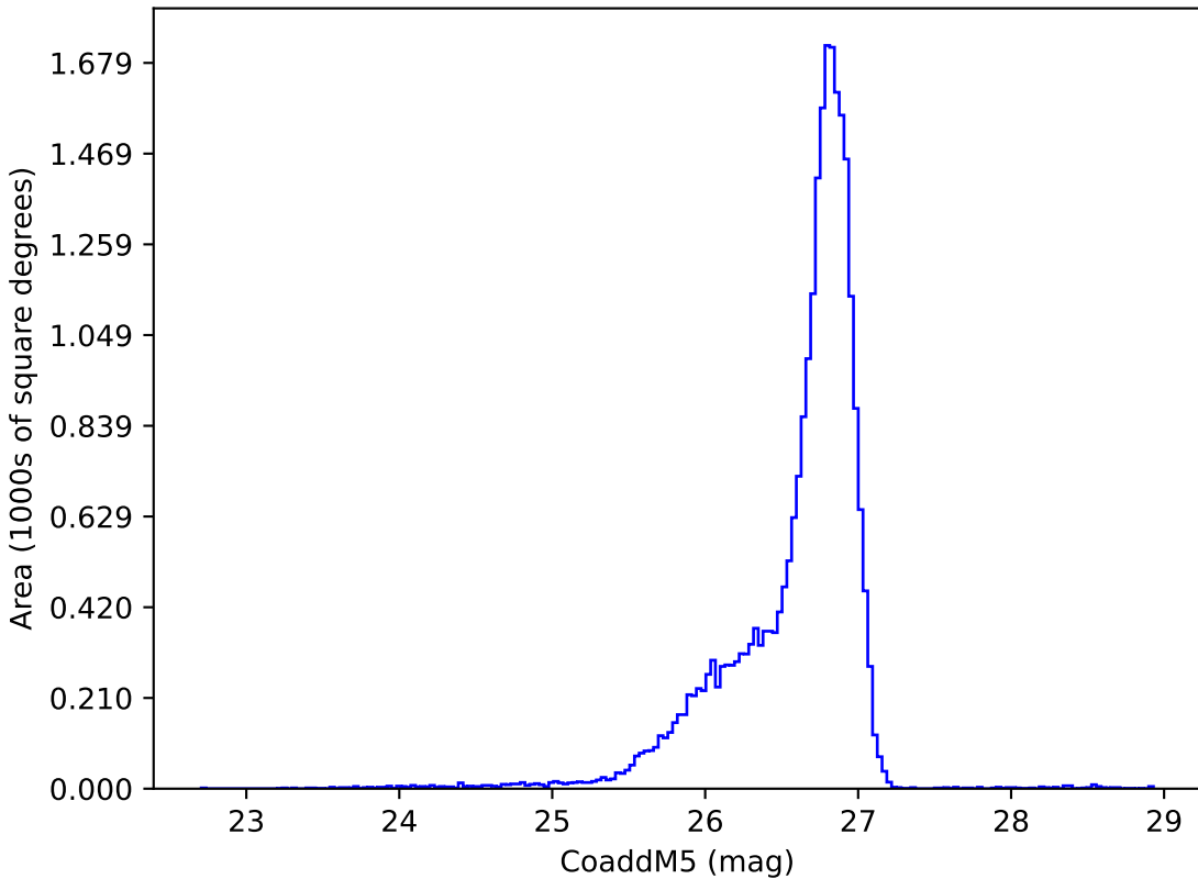
too_elab_r256_d2_ugrizy_v3.4_10yrs g: CoaddM5
