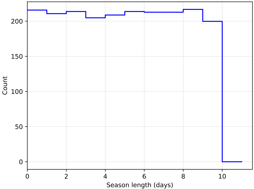
too_elab_r256_d2_ugrizy_v3.4_10yrs DD:ECDFS all bands: SeasonLength
