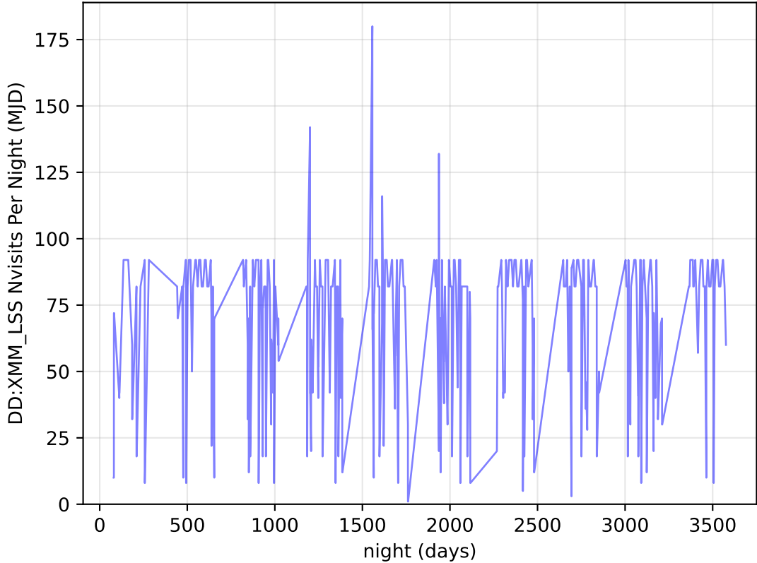
too_elab_r256_d2_ugrizy_v3.4_10yrs all bands: DD:XMM_LSS Nvisits Per Night
