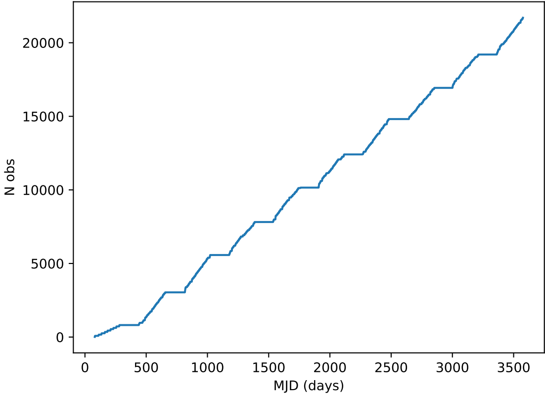
too_elab_r256_d2_ugrizy_v3.4_10yrs all bands: DD:XMM_LSS Cumulative NVisits
