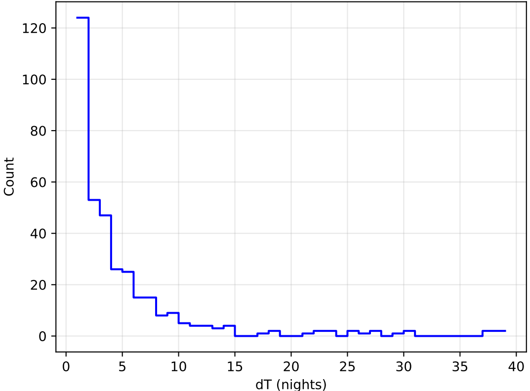
too_elab_r256_d2_ugrizy_v3.4_10yrs all bands: DD:WFD Delta Nights Histogram
