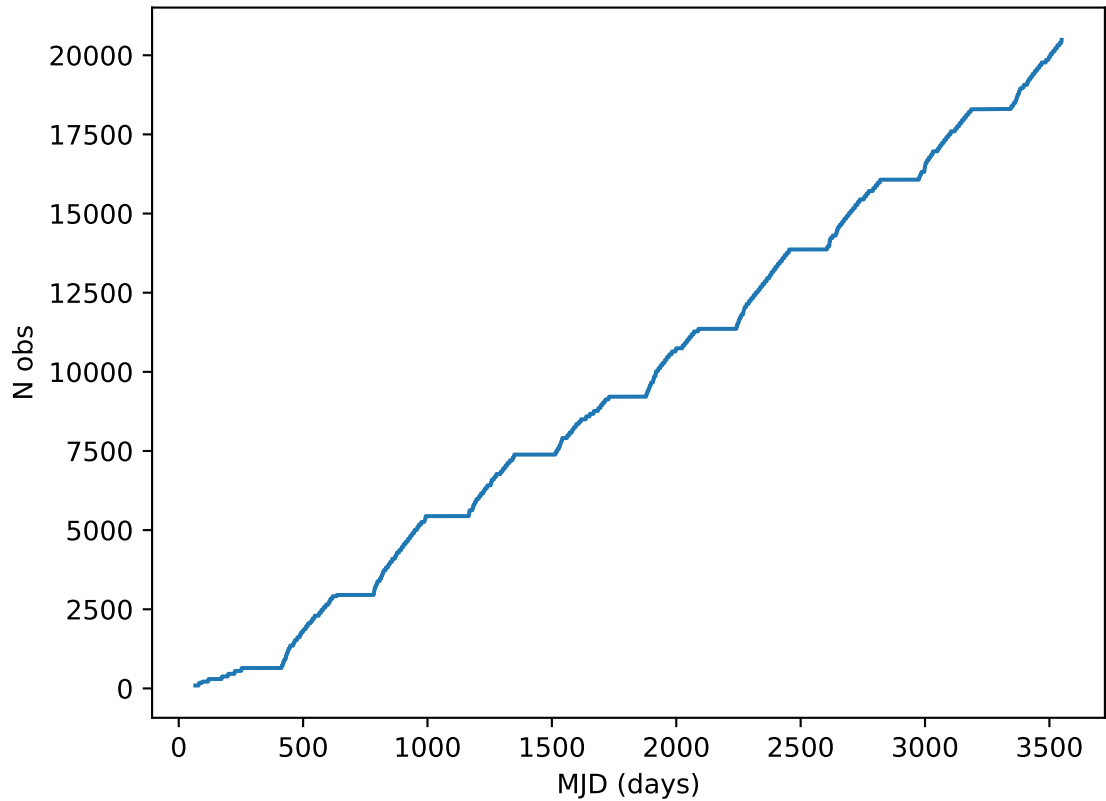
too_elab_r256_d2_ugrizy_v3.4_10yrs all bands: DD:ELAISS1 Cumulative NVisits
