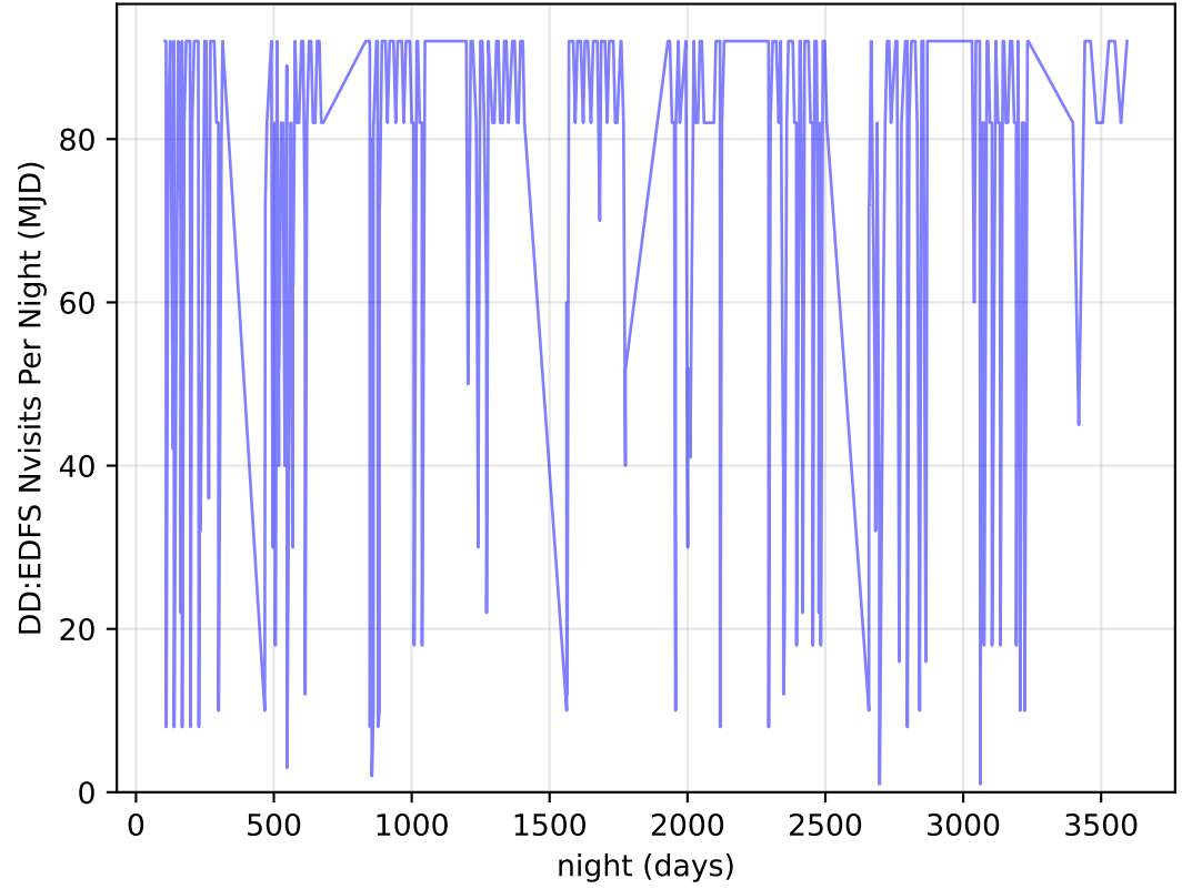
too_elab_r256_d2_ugrizy_v3.4_10yrs all bands: DD:EDFS Nvisits Per Night
