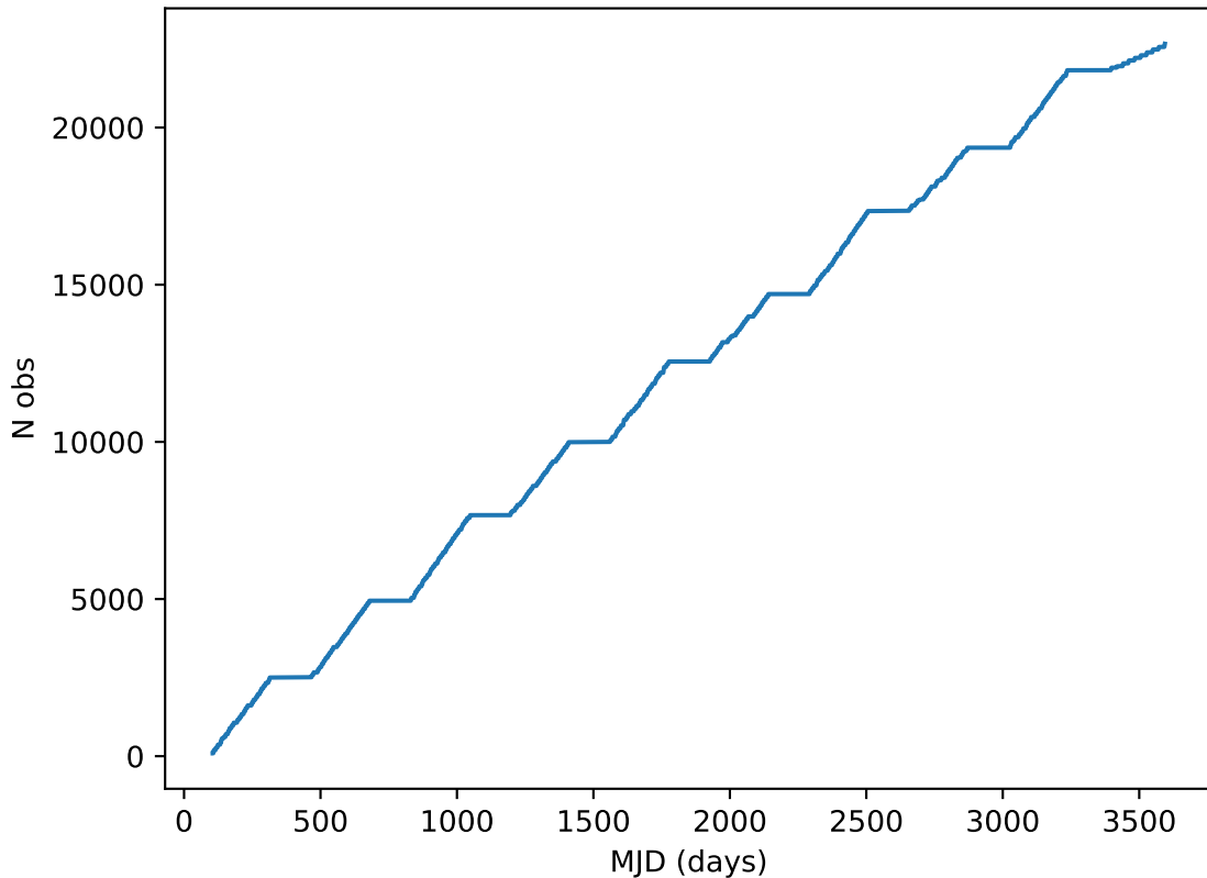
too_elab_r256_d2_ugrizy_v3.4_10yrs all bands: DD:EDFS Cumulative NVisits
