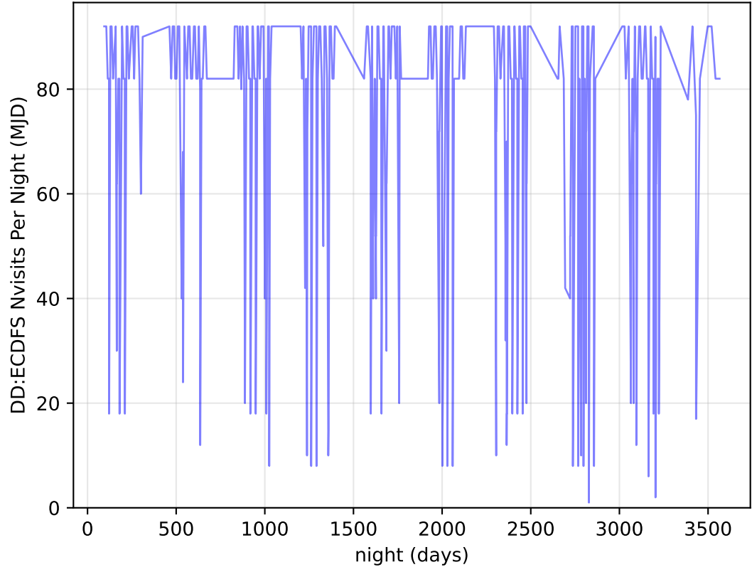
too_elab_r256_d2_ugrizy_v3.4_10yrs all bands: DD:ECDFS Nvisits Per Night
