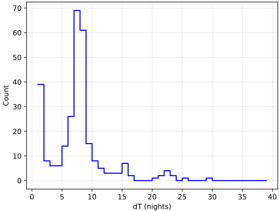
too_elab_r256_d2_ugrizy_v3.4_10yrs all bands: DD:ECDFS Delta Nights Histogram
