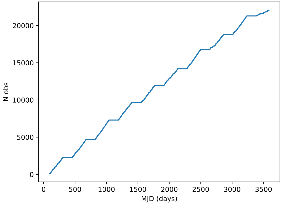
too_elab_r256_d2_ugrizy_v3.4_10yrs all bands: DD:ECDFS Cumulative NVisits
