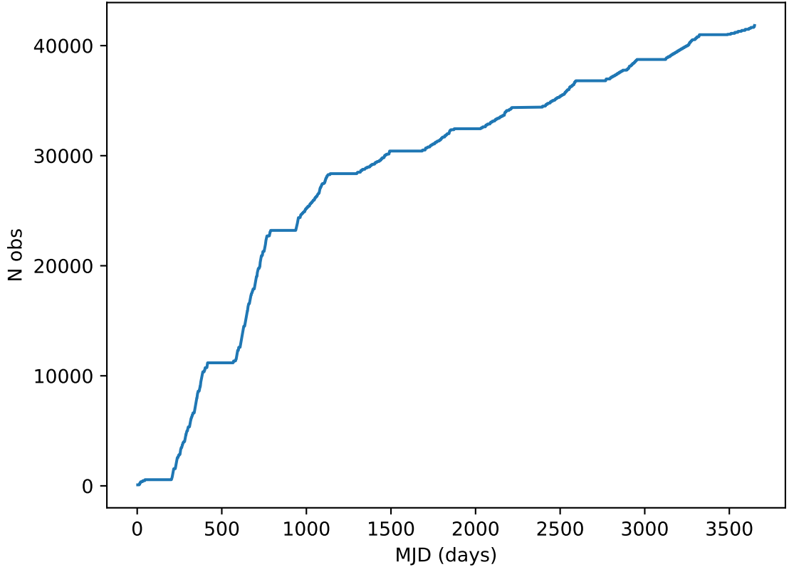
too_elab_r256_d2_ugrizy_v3.4_10yrs all bands: DD: COSMOS Cumulative NVisits
