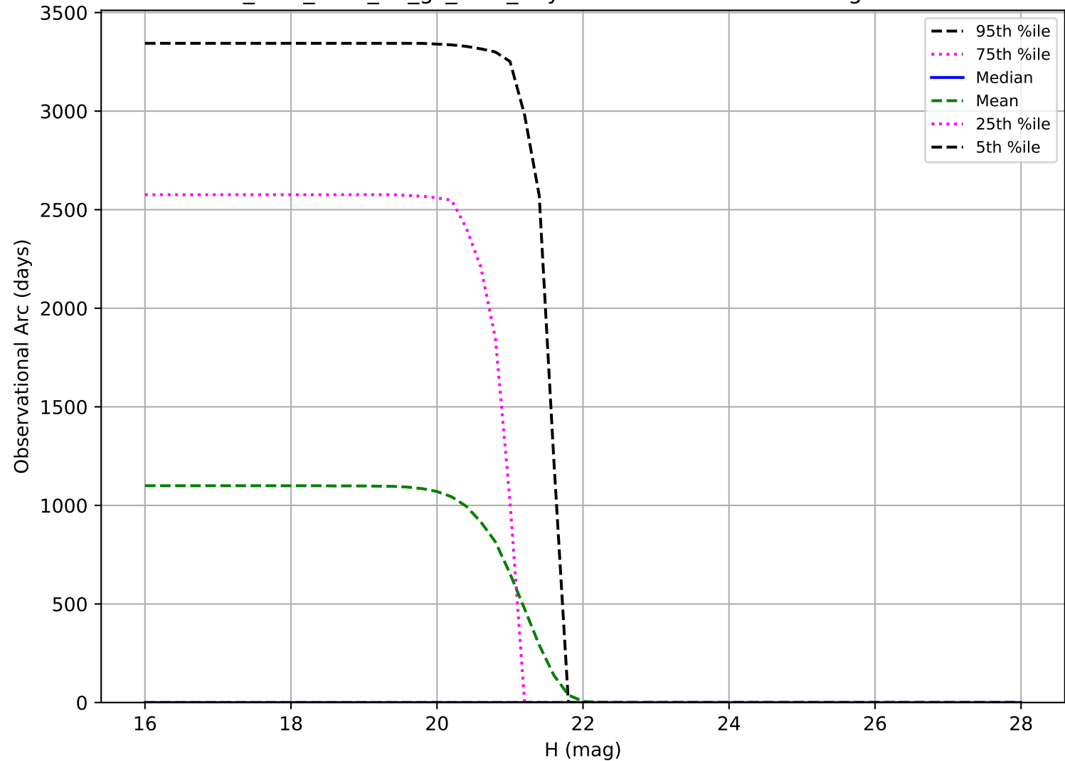
too_elab_r256_d2_gz_v3.4_10yrs: Observational Arc Length Vatira
