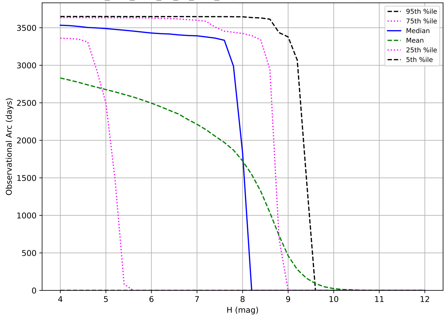
too_elab_r256_d2_gz_v3.4_10yrs: Observational Arc Length TNO
