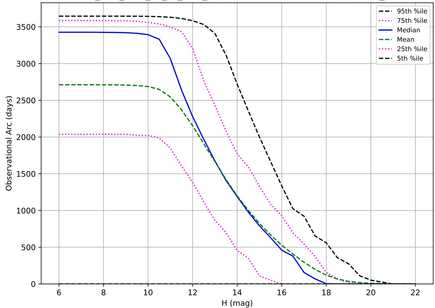
too_elab_r256_d2_gz_v3.4_10yrs: Observational Arc Length OCC_r5
