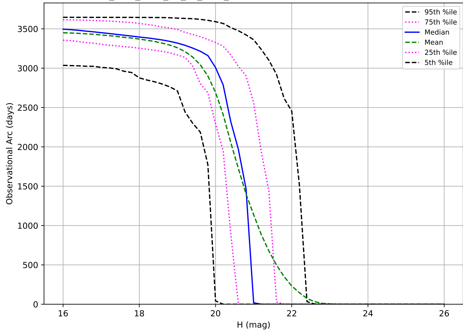
too_elab_r256_d2_gz_v3.4_10yrs: Observational Arc Length MBA
