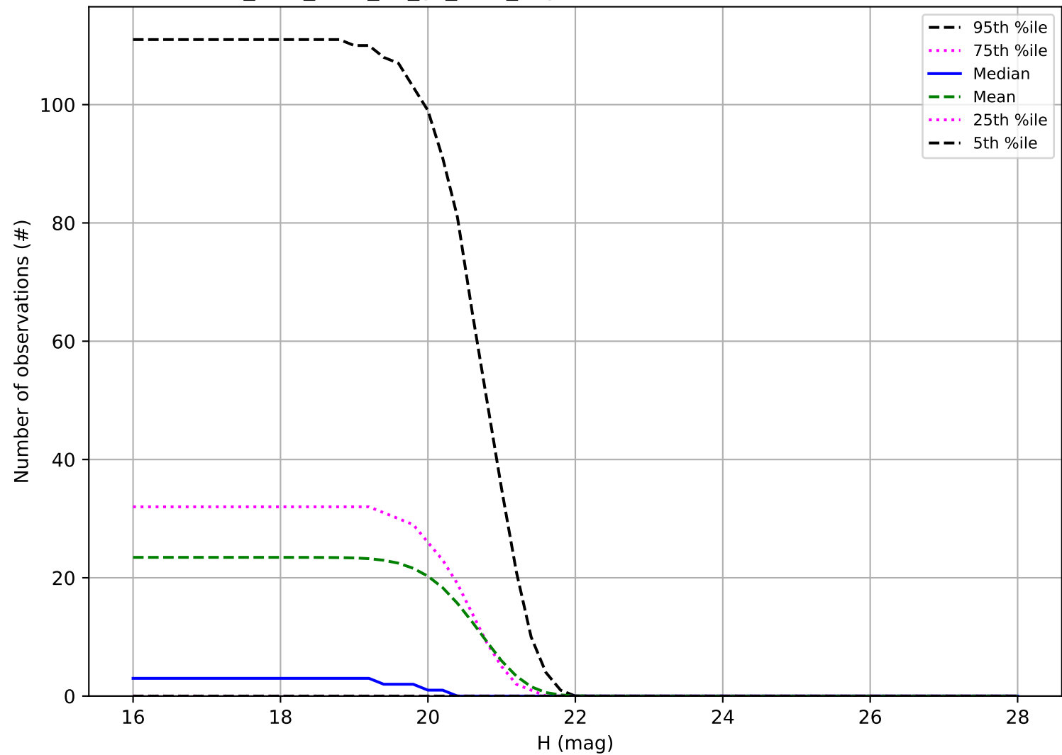
too_elab_r256_d2_gz_v3.4_10yrs: Number of observations Vatira
