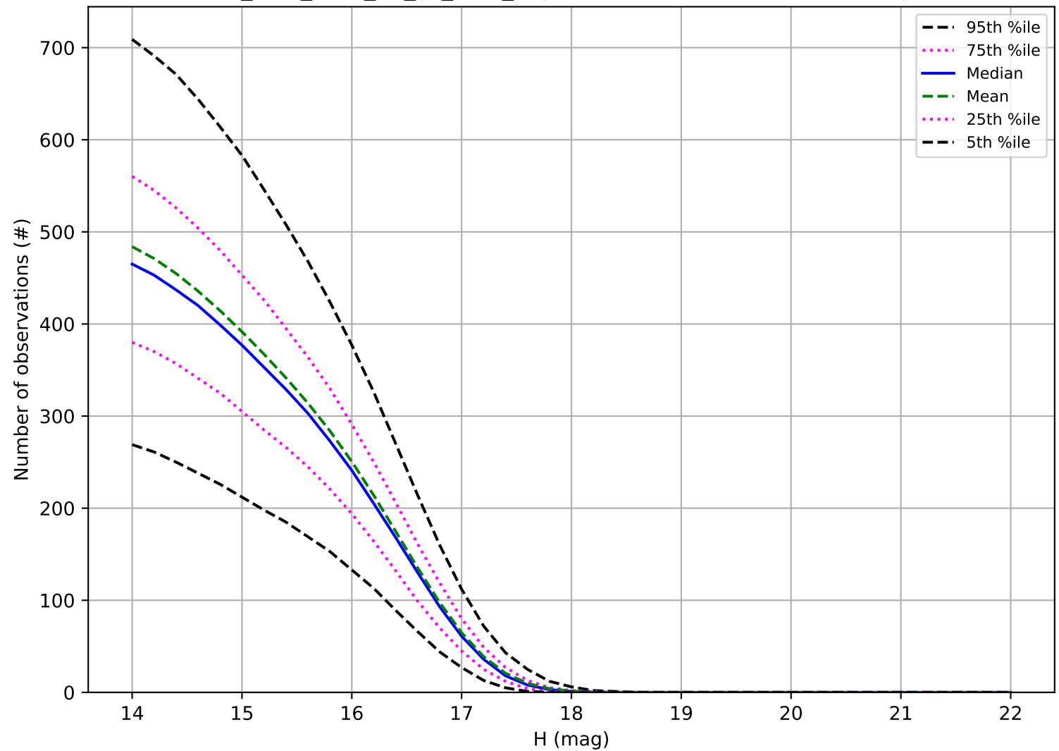
too_elab_r256_d2_gz_v3.4_10yrs: Number of observations Trojan
