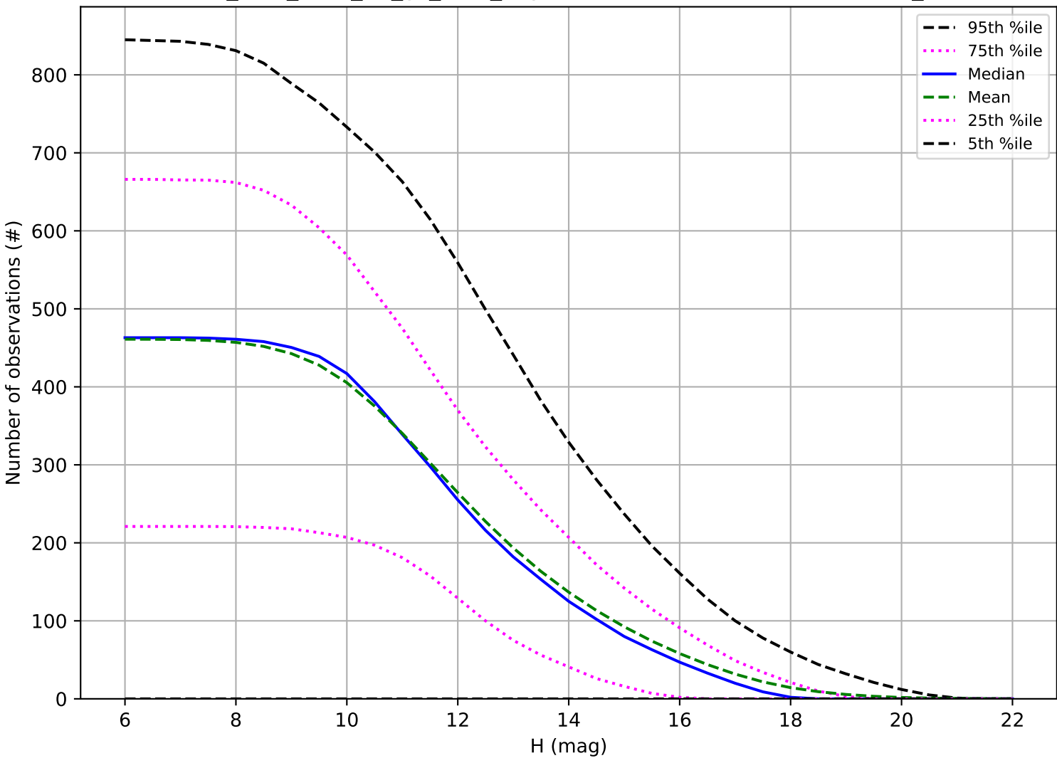
too_elab_r256_d2_gz_v3.4_10yrs: Number of observations OCC_r5
