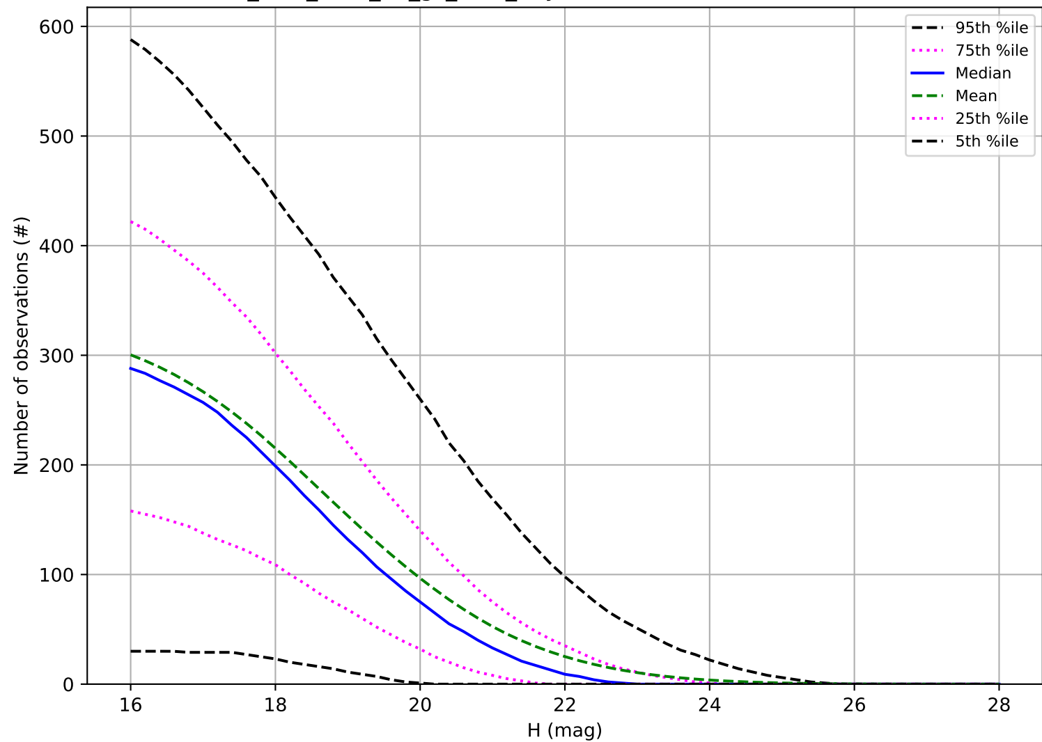
too_elab_r256_d2_gz_v3.4_10yrs: Number of observations NEO
