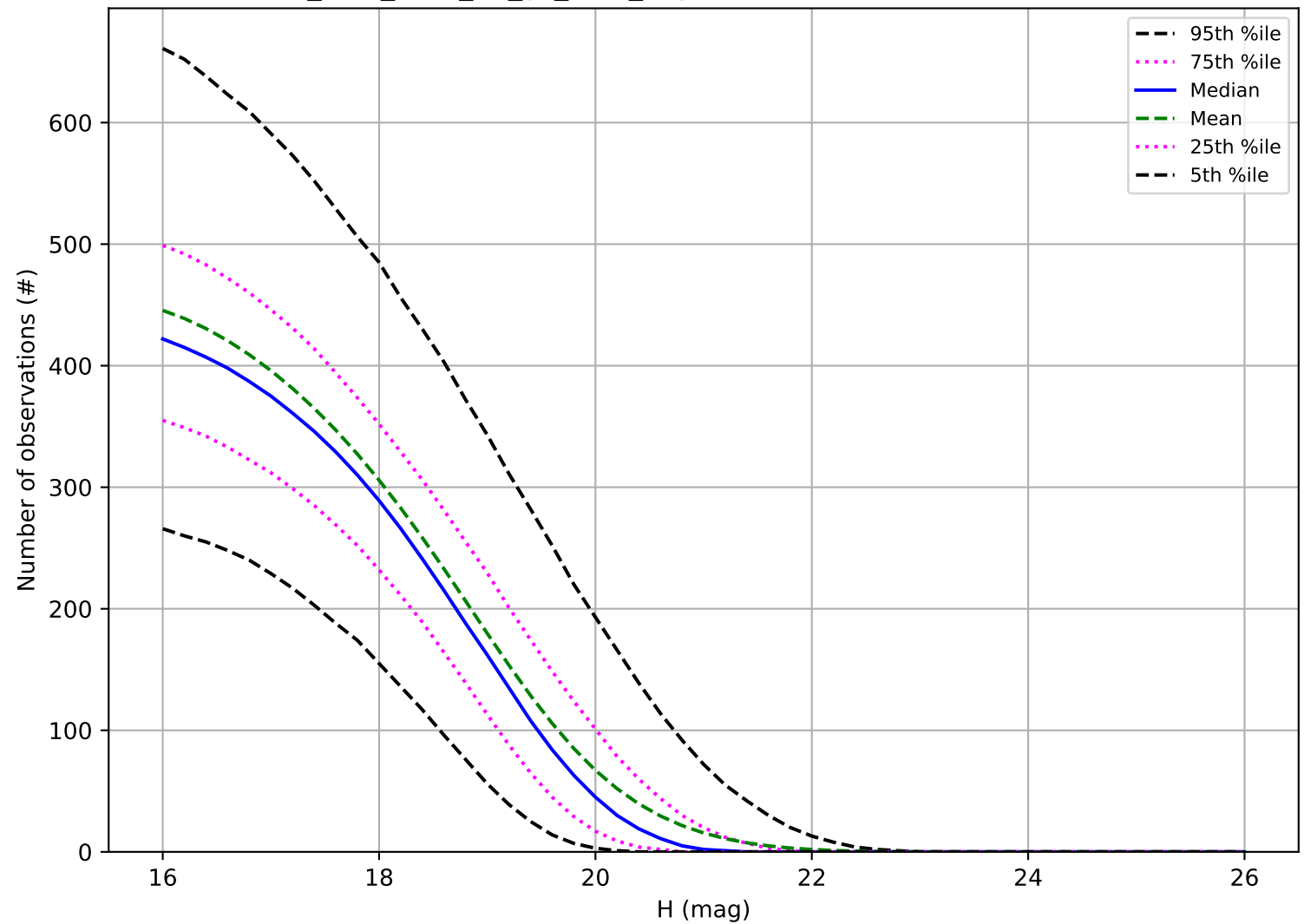
too_elab_r256_d2_gz_v3.4_10yrs: Number of observations MBA
