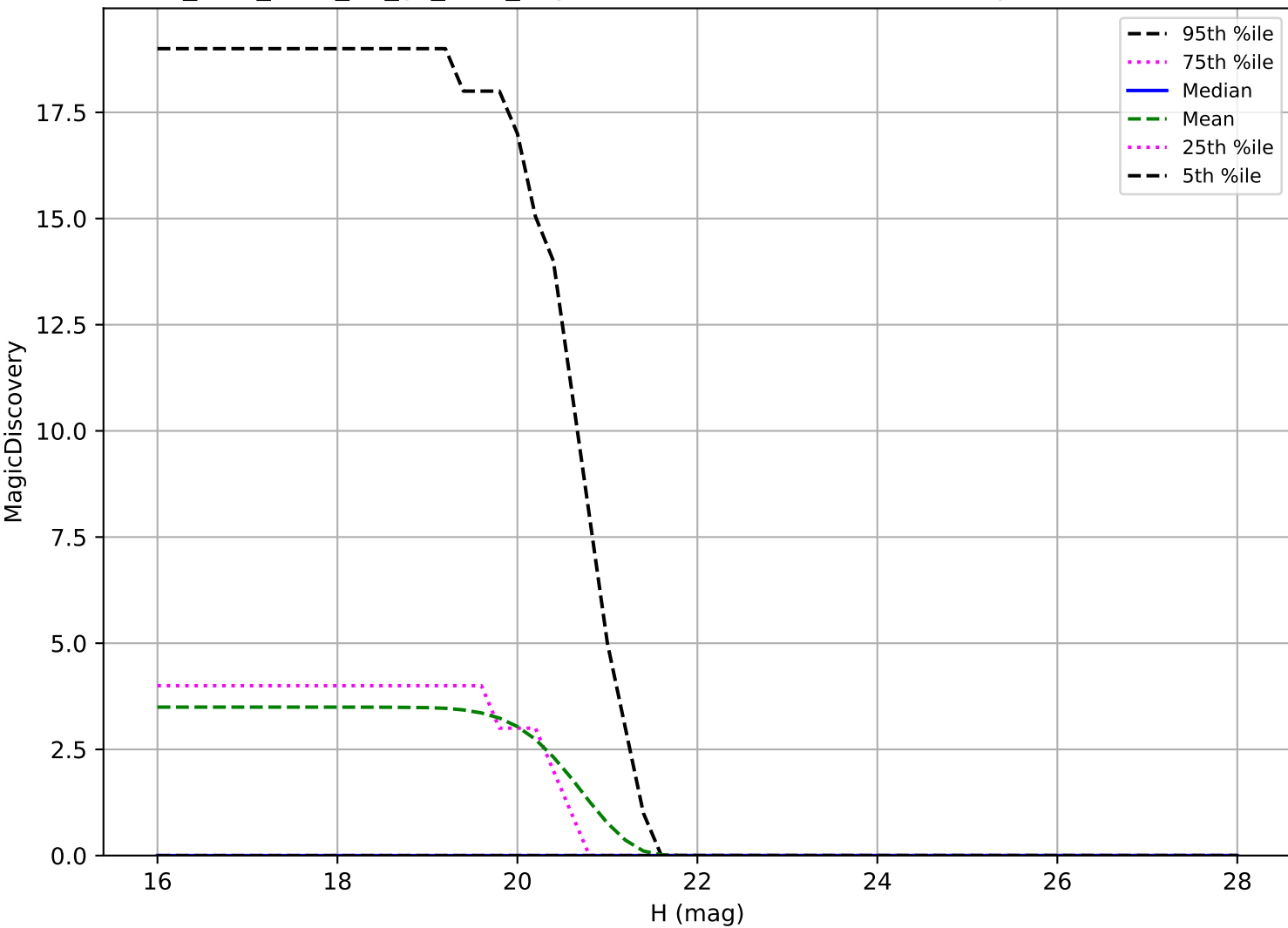
too_elab_r256_d2_gz_v3.4_10yrs: Vatira 6 detections in 60 nights detection loss
