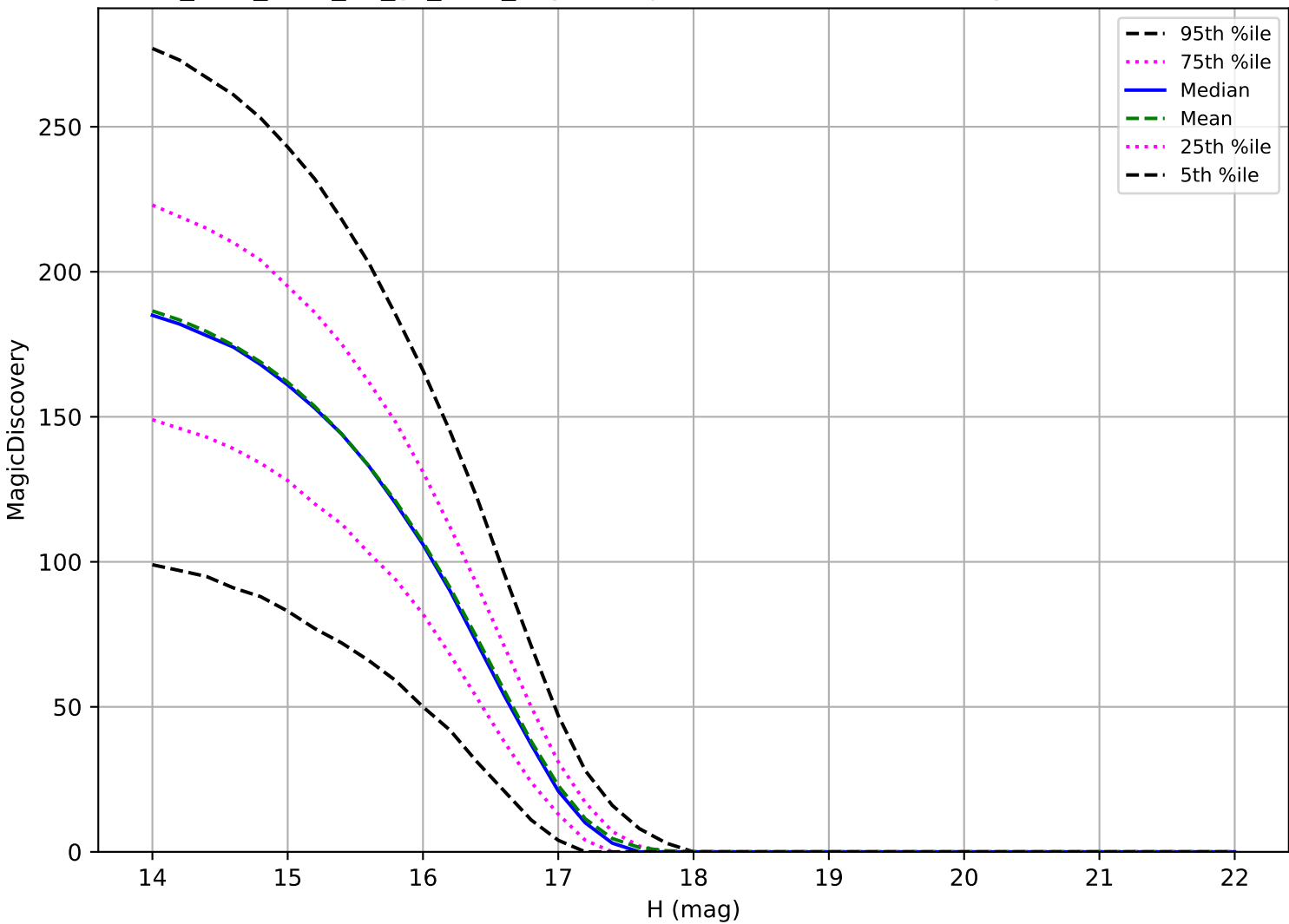
too_elab_r256_d2_gz_v3.4_10yrs: Trojan 6 detections in 60 nights detection loss
