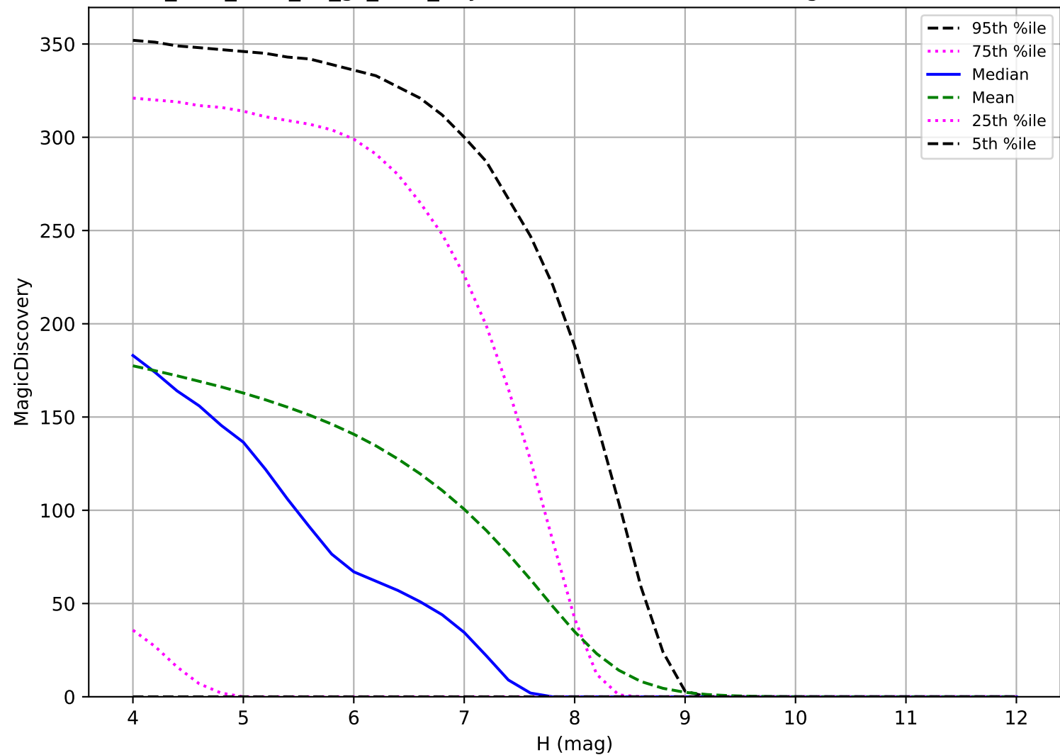
too_elab_r256_d2_gz_v3.4_10yrs: TNO 6 detections in 60 nights detection loss
